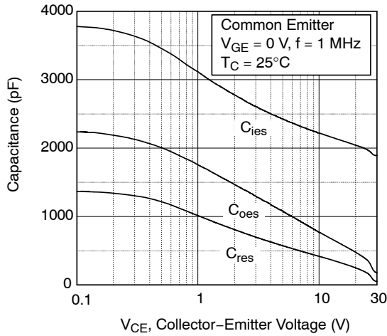
Figure 9. Capacitance Characteristics
