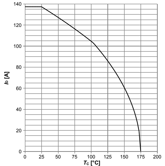
Diagram 2: Drain current
