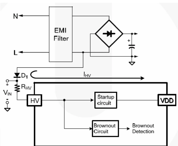
Figure 5. Brownout Circuit
