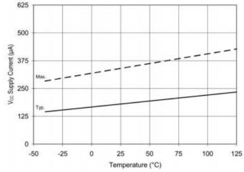
Figure 18A. V CC Supply Current vs. Temperature
